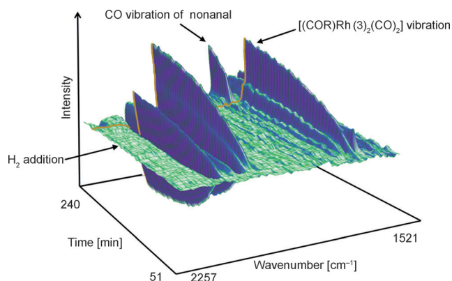
Figure 5. Difference in situ IR spectra obtained after the addition of 1.5 equiv 1-octene under CO pressure to the solution of the [\text{HRh}(\text{PPh}_2)_3(\text{CO})_2] complex ( 10^{-2} M in toluene). The orange line marks the addition of \text{H}_2 .
