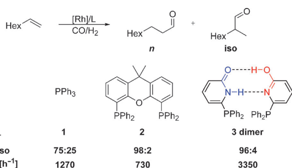
Scheme 1. Selectivity and activity observed in the rhodium-catalyzed hydroformylation of 1-octene with various ligands. Conditions: \text{Rh}/\text{L}/\text{substrate} = 1:20(10):7500 , 80^\circ\text{C} , 10 bar, toluene.
